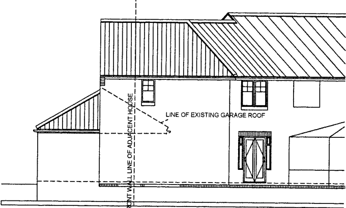
REAR ELEVATION
